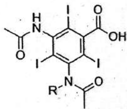
diatrizoic acid (R = H)
