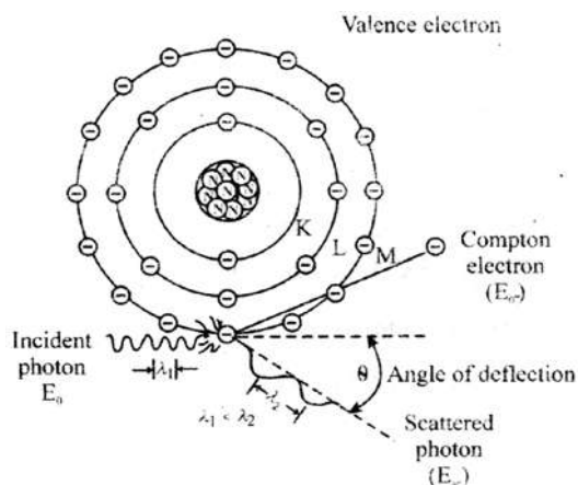
Fig. 2.8.4: Compton Scattering
