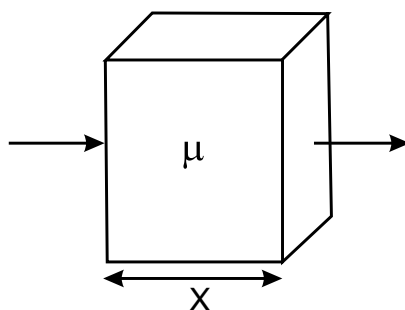
Fig. 2.8.1: Radiation Attenuation.
