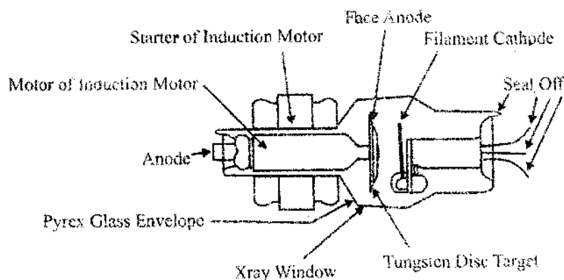
Fig. 2.7.5: Rotating Anode X-Ray Tube
