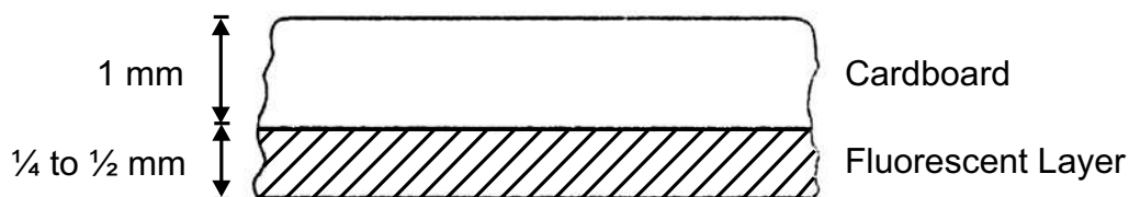
Fig. 4.3.1: Intensifying Screen
