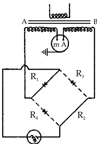
Fig. 2.6.4: Circuit for full wave rectification
